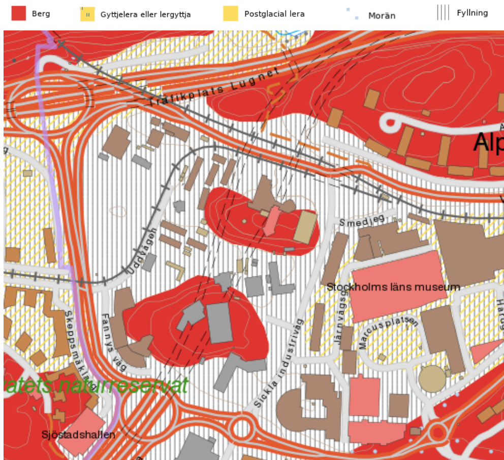
Figur 4. SGUs jordartskarta, skala 1:25000.
